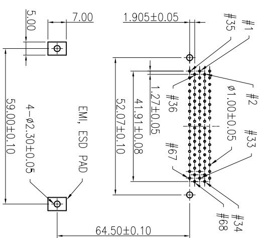
RECOMMENDED HOLE PATTERN
